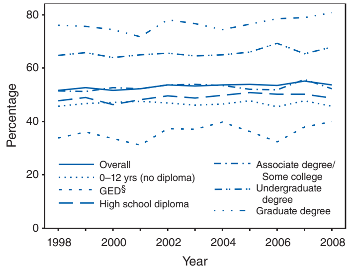
FIGURE 2. Quit ratios* among former smokers † aged \geq 25 years, by education — National Health Interview Survey, United States, 1998–2008
